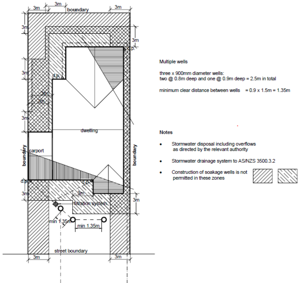
Figure B2 - Location of soakage wells
