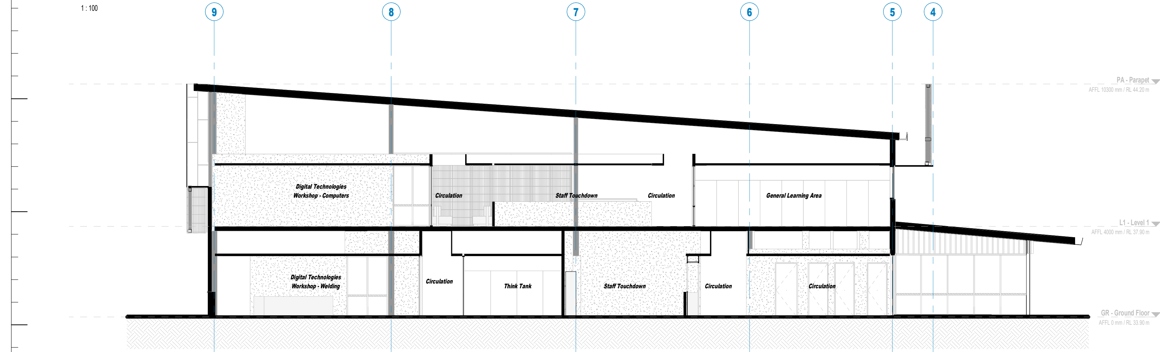
Section A 1:100
