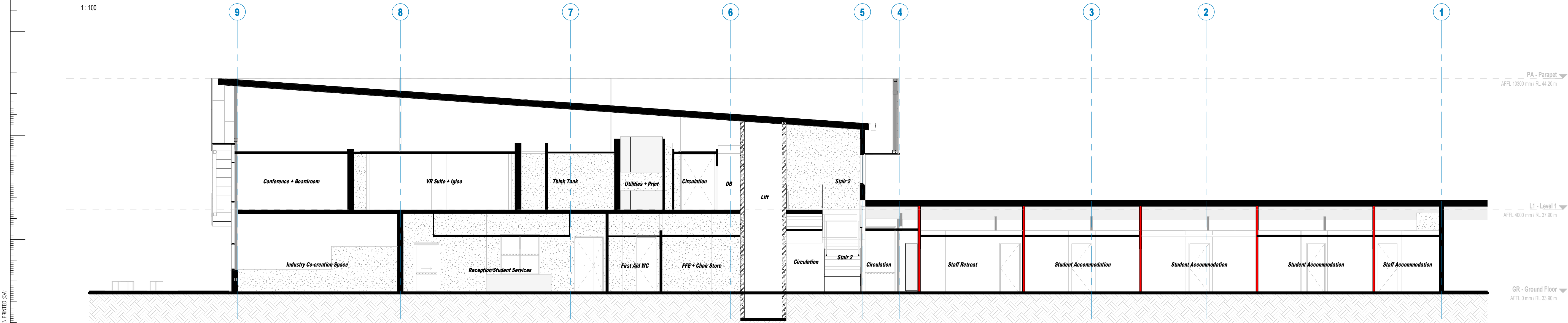
Section C 1:100
